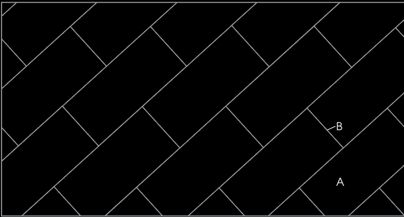
BROKEN BOND 304.8 x 457.2 mm Stripping optional: 3.2 x 914.4 mm
